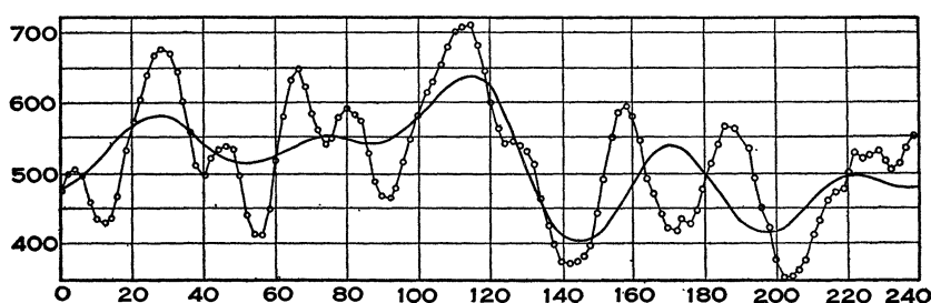
FIGURE 8.—o-o-o The first 120 even terms of Model II. — Sum of the first five harmonics of Fourier series: y = 518.14 - 20.98 \cos (2\pi t/240) + 50.02 \sin (2\pi t/240) + 17.30 \cos (2\pi t/120) - 3.16 \sin (2\pi t/120) - 10.93 \cos (2\pi t/80) + 35.66 \sin (2\pi t/80) + 17.18 \cos (2\pi t/60) - 21.92 \sin (2\pi t/60) - 38.53 \cos (2\pi t/48) - 3.65 \sin (2\pi t/48) .
